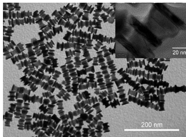
Figure 4. A typical TEM image of complex \text{Cu}_{1.94}\text{S} - \text{ZnS} - \text{Cu}_{1.94}\text{S} - \text{ZnS} - \text{Cu}_{1.94}\text{S} sandwich-like heteronanostructures prepared by using \text{CuI} and [\text{Zn}(\text{S}_2\text{CNEt}_2)_2] as precursors with a molar ratio of 13:8. Inset: a high-resolution TEM image of a typical example of such a heteronanostructure.
